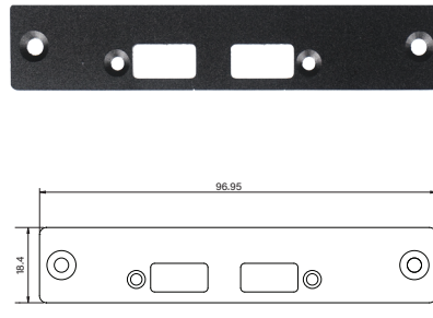
UB1314 Universal Bracket with 2x USB Cutout Dimension (WxD): 96.95 x 18.4 mm
