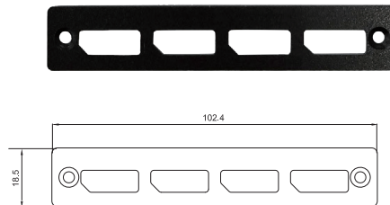
UB1329 Universal Bracket with 4x DP Cutout Dimension (WxD): 102.4 x 18.5 mm
