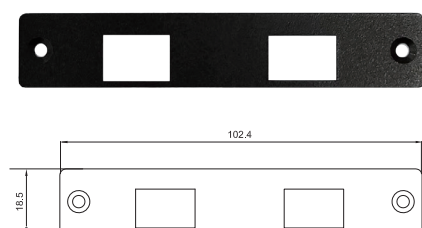
UB1328 Universal Bracket with 2x RJ45 Cutout Dimension (WxD): 102.4 x 18.5 mm
